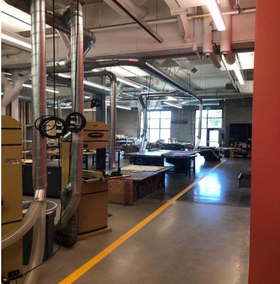
CVHS Building F – Wood shop with dust collector and power connected
