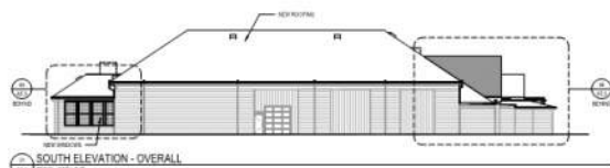
SOUTH ELEVATION - OVERALL SCALE: 1/8" = 1'-0"
