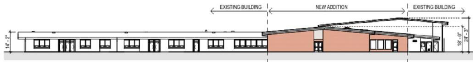
EAST ELEVATION
