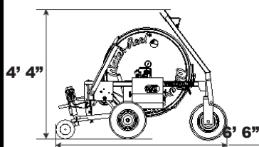
Sprinkler Diagram
