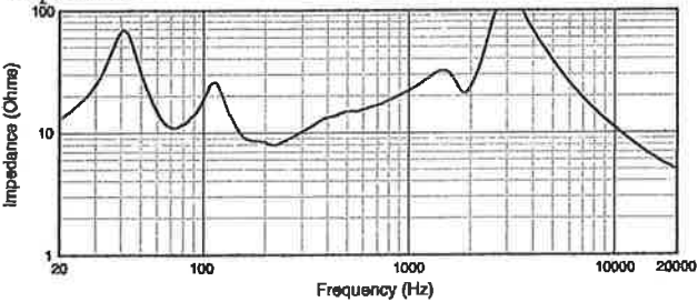
Impedance
