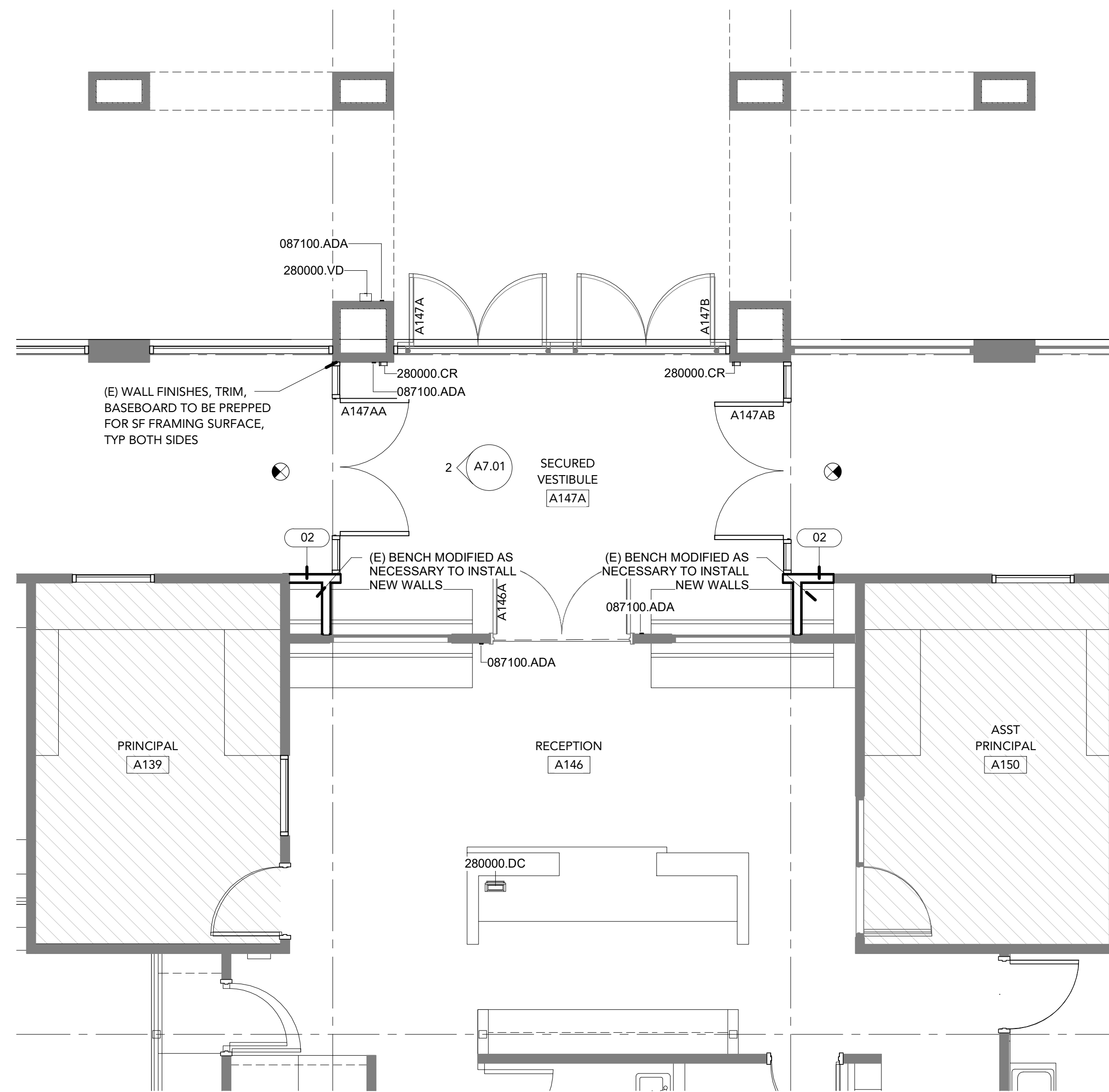
1 ENLARGED FLOOR PLAN - MAIN OFFICE 1/4" = 1'-0"
