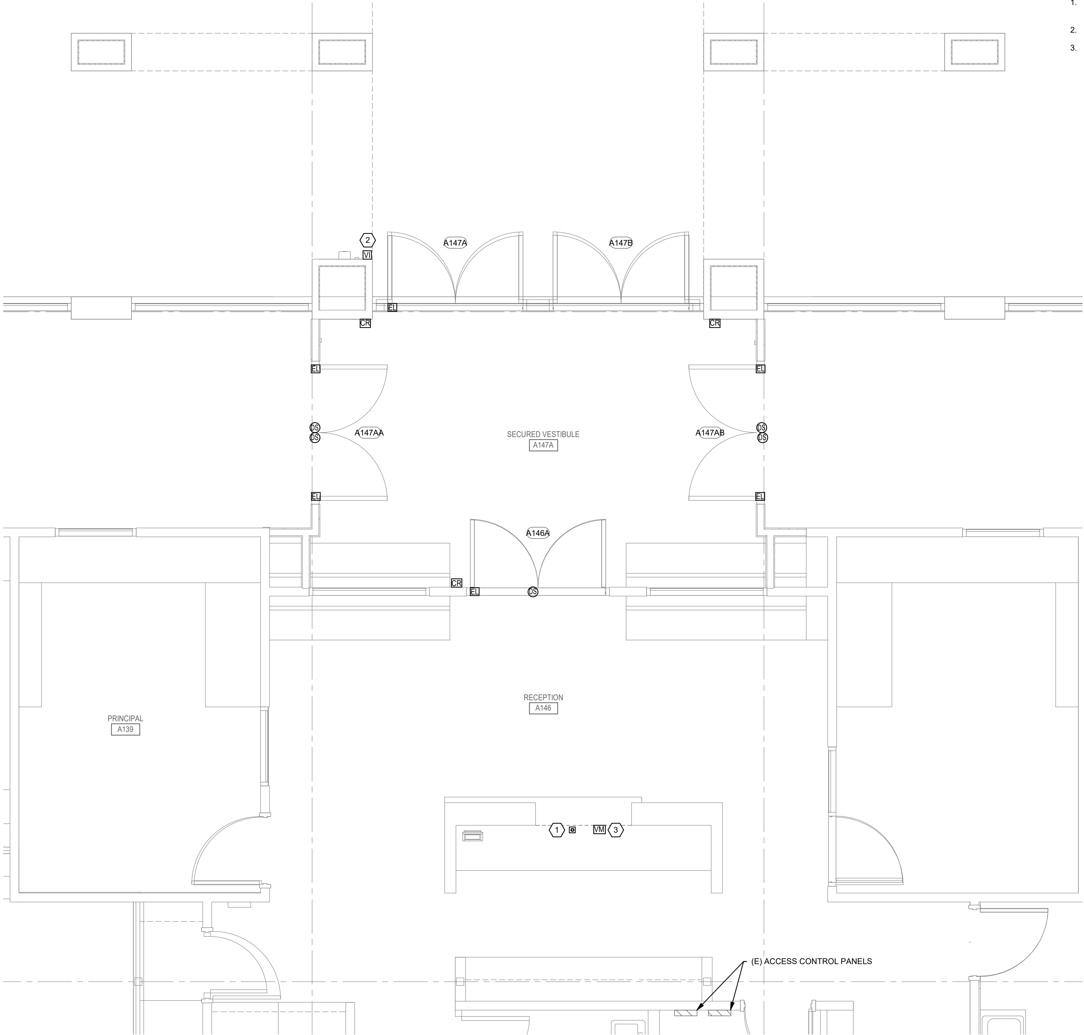
1 ENLARGED FLOOR PLAN - MAIN OFFICE - TECHNOLOGY
