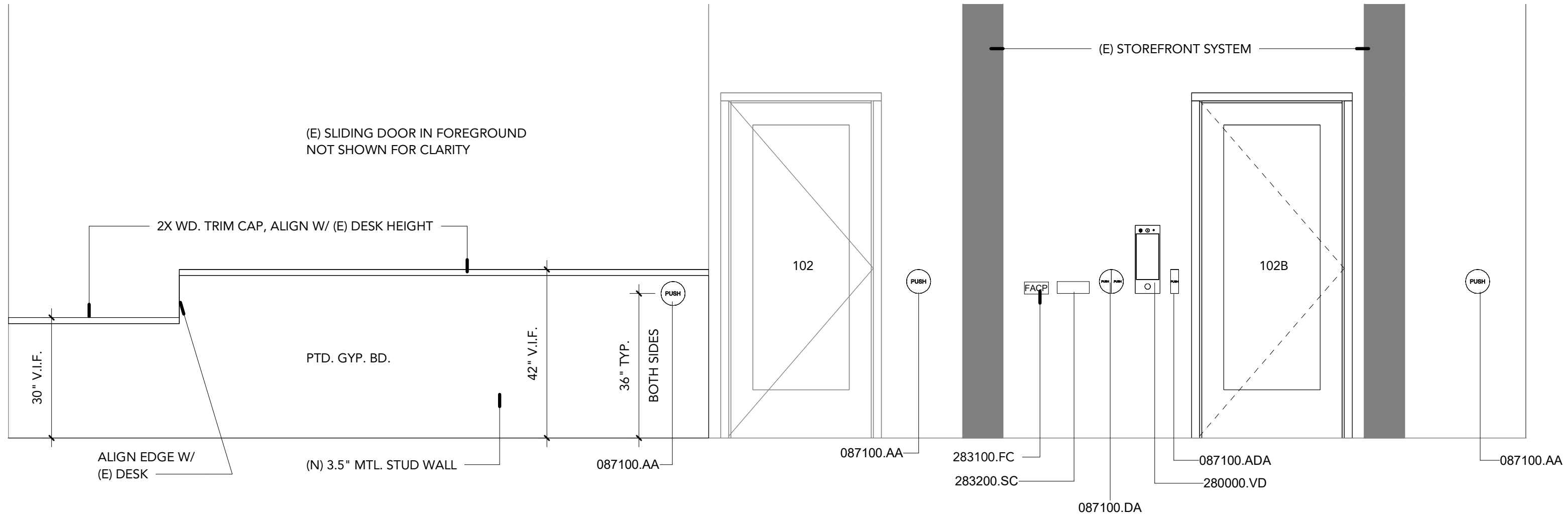
3 SOUTH WALL VESTIBULE AND OFFICE ENTRY 1/2" = 1'-0"
