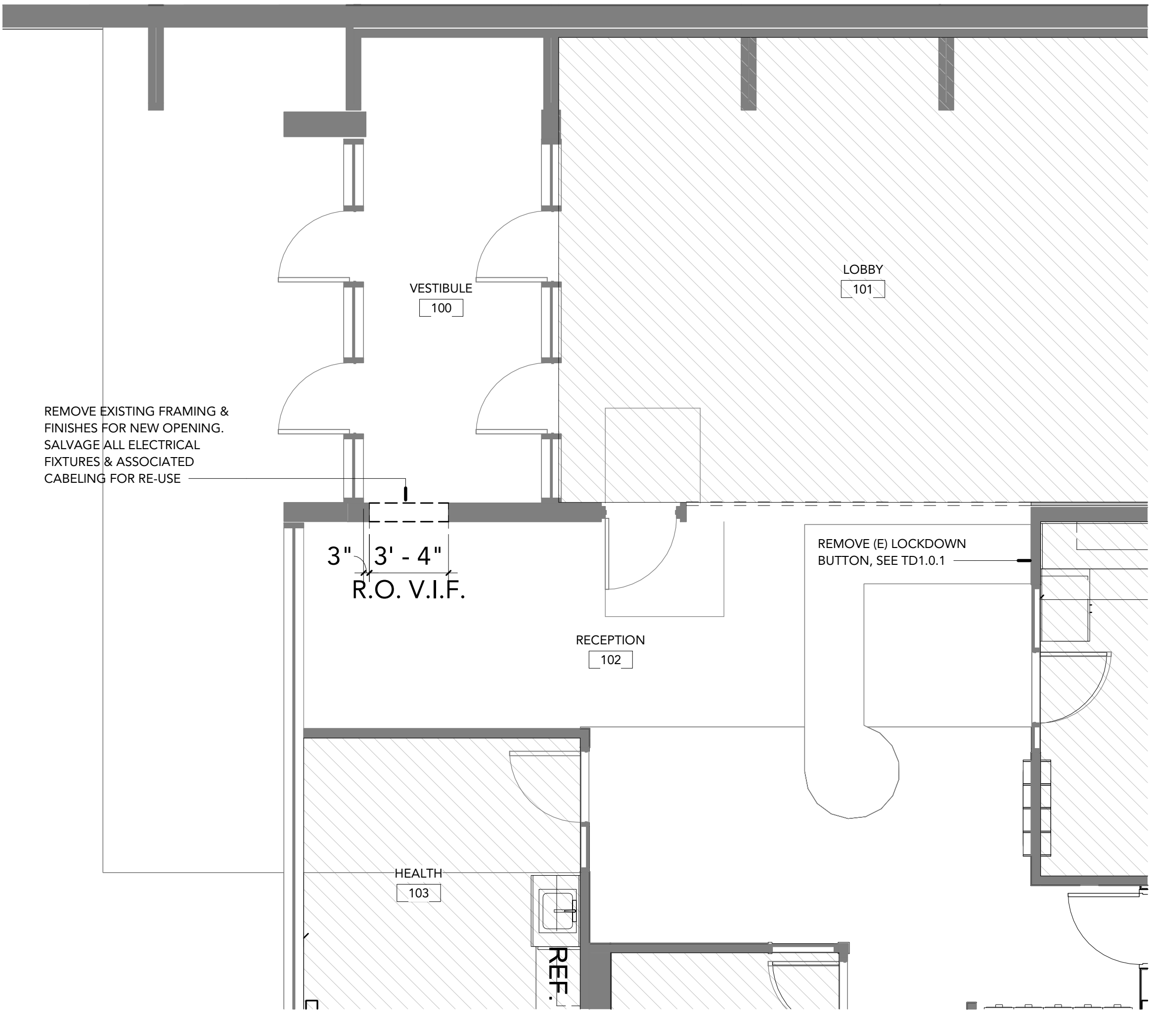
1 DEMOLITION PLAN - SECURED VESTIBULE 1/4" = 1'-0"
