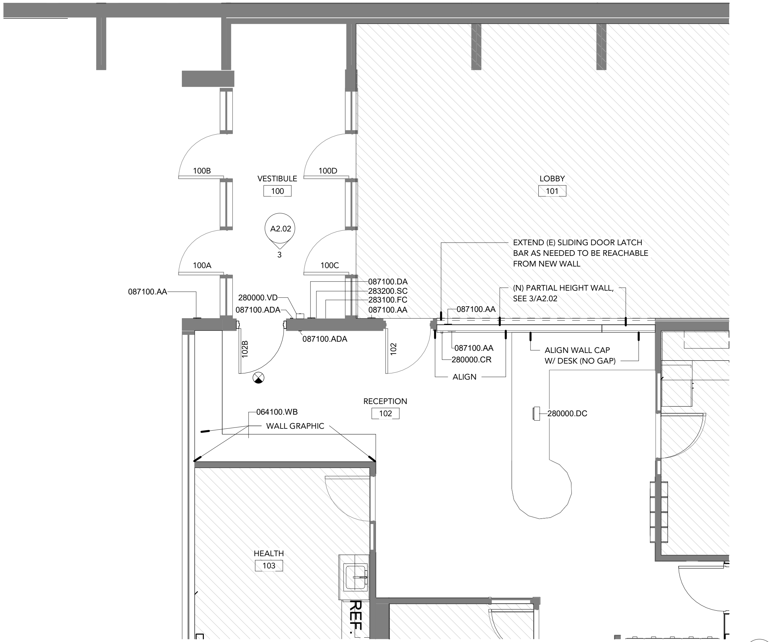
2 ENLARGED PLAN - SECURED VESTIBULE 1/4" = 1'-0"
