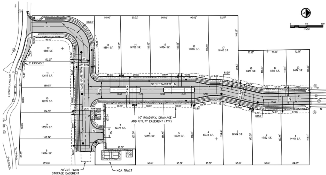
Site Plan
