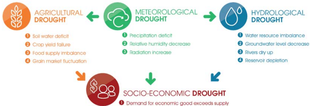
Figure 46: Drought Transfer Process and Interactions
