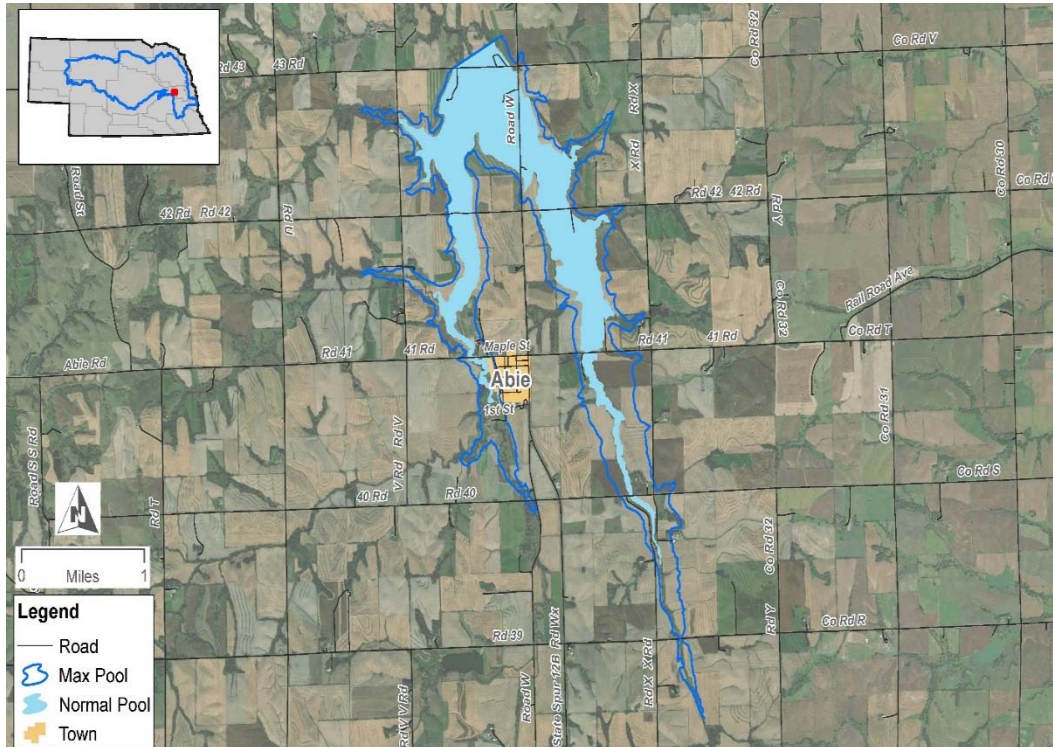
Figure 52: Skull Creek Reservoir Proposed Location
