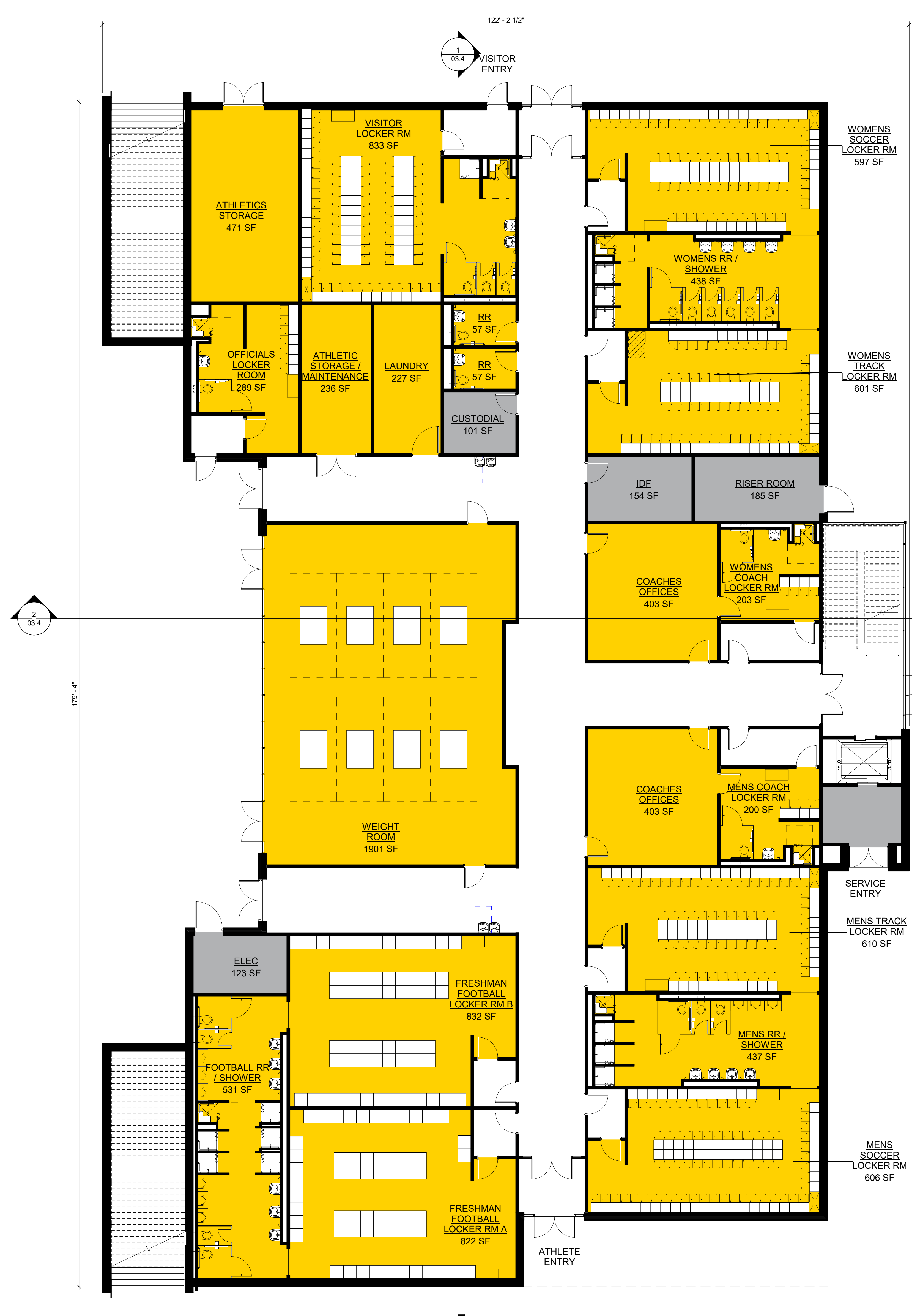
FLOOR PLAN - LEVEL ONE
