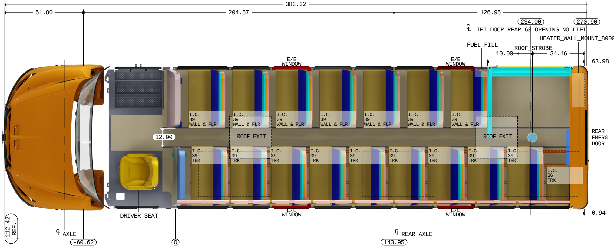
HIP-TO-KNEE SPACING (INCHES)+/-0.5"
